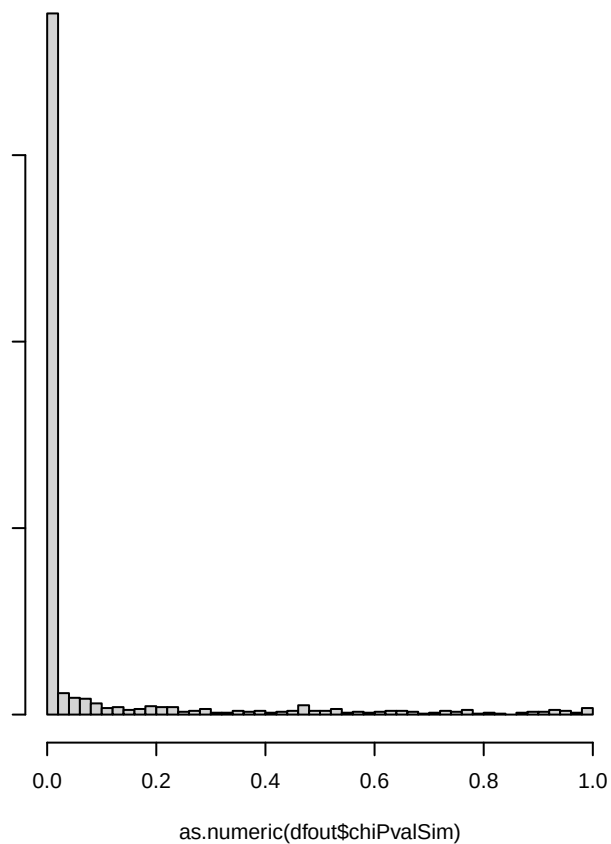
chisq SimPval distribution, numsig: 784 /1000
